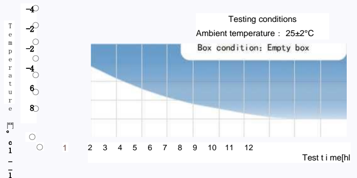
CPF10L80 Portable Cryogenic Freezer Refrigeration curve
